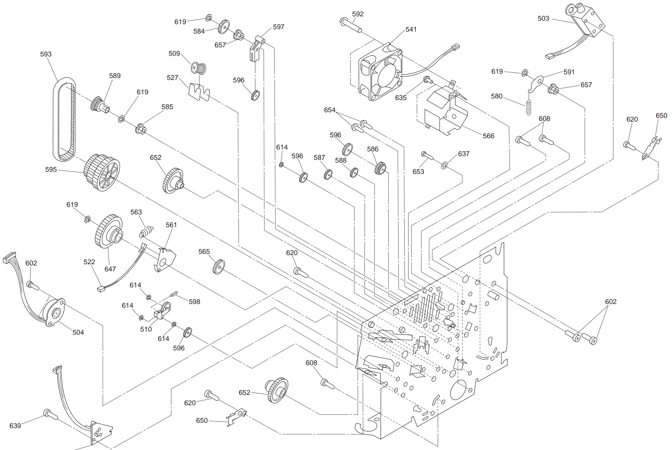
EXPLODED DIAGRAM FOR DFX-8500(7)
