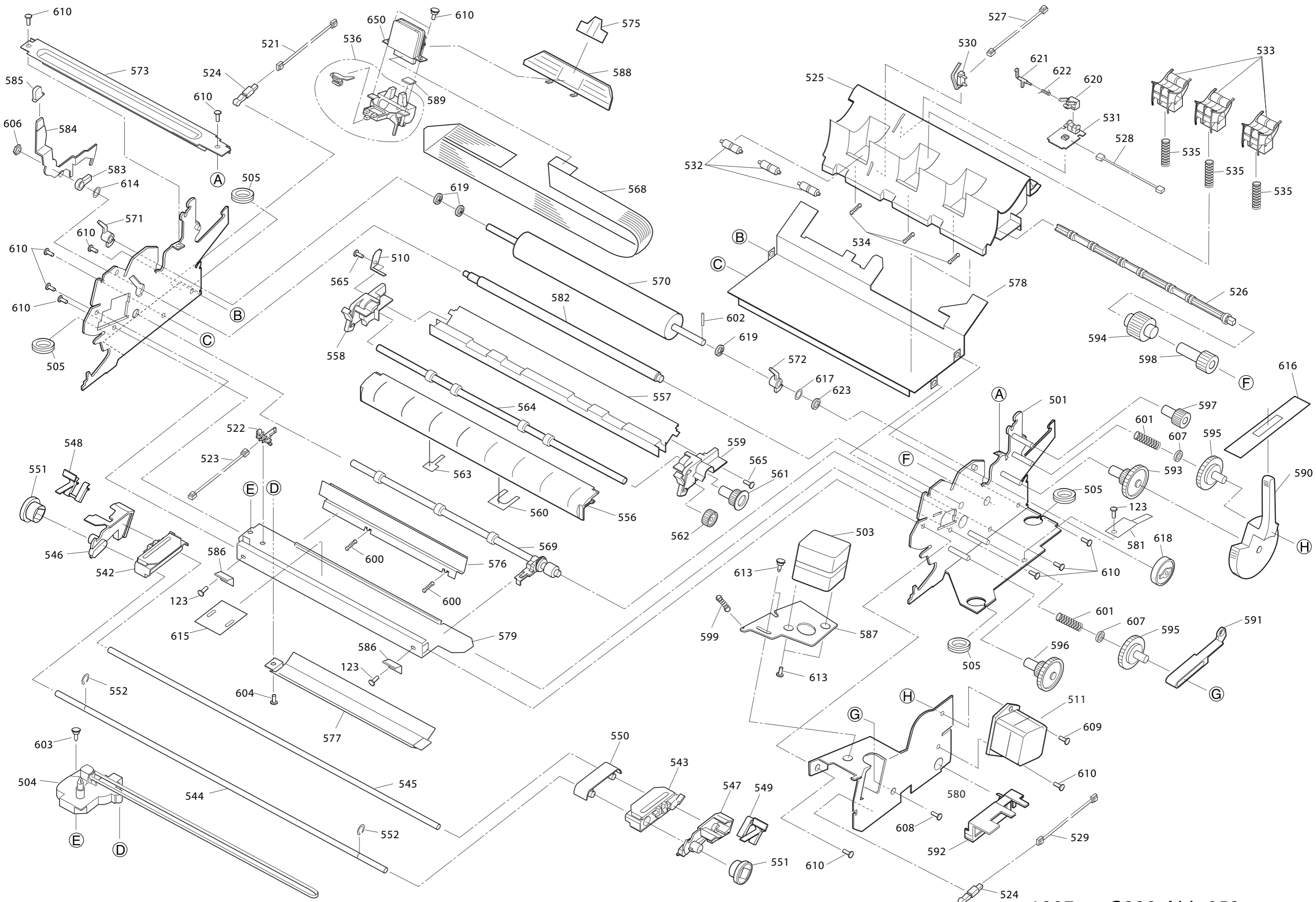
EXPLODED DIAGRAM FOR FX-880(2)
