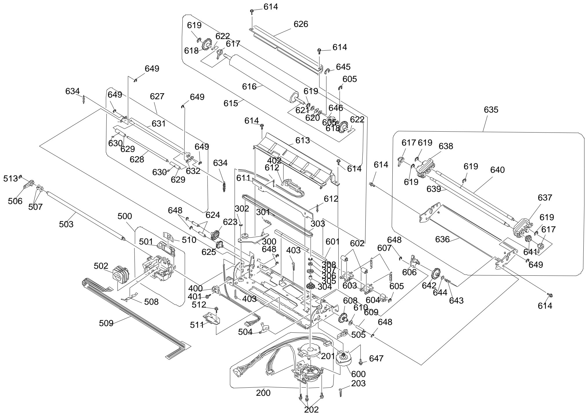
EXPLODED DIAGRAM FOR M-2000
