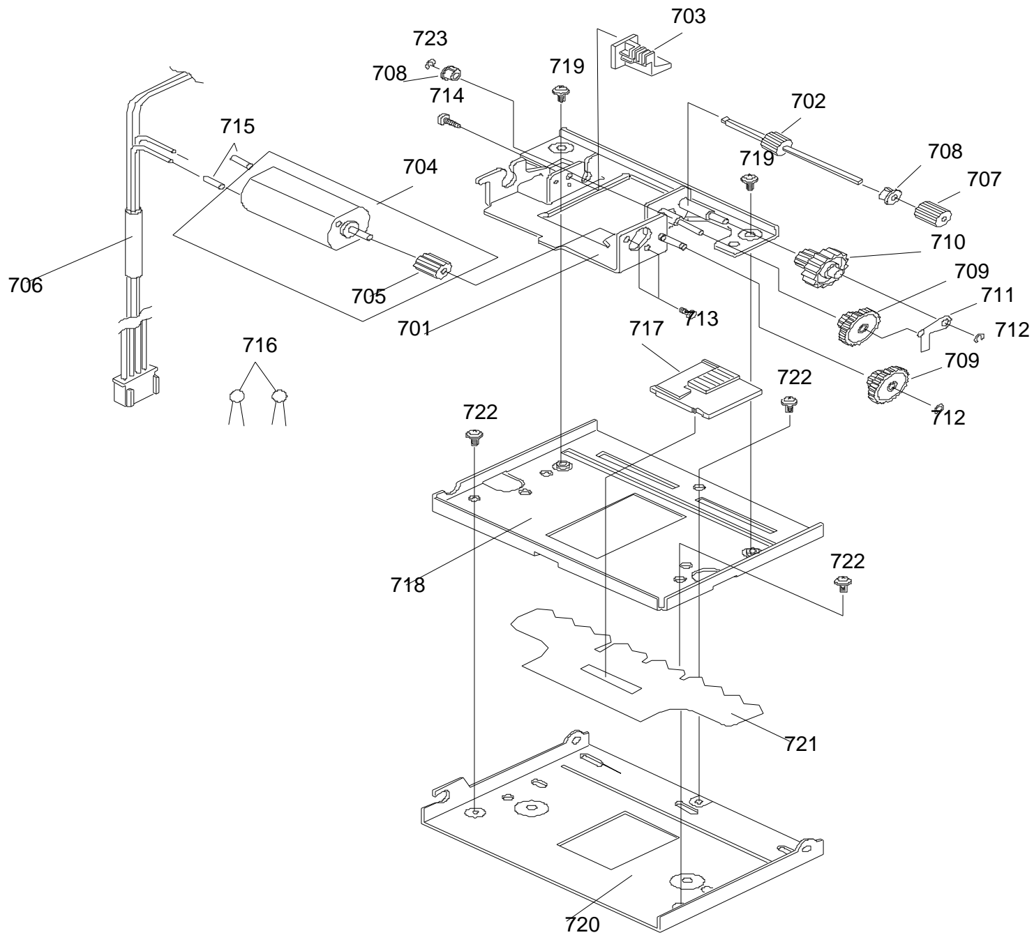
EXPLODED DIAGRAM FOR TM-U300A/U300B/U300PA/U300PB (AUTO CUTTER UNIT)
